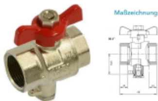
Sensus WMZ Kugelhahn-Set DN25 L:66 IG1" PN16 45/5,2
